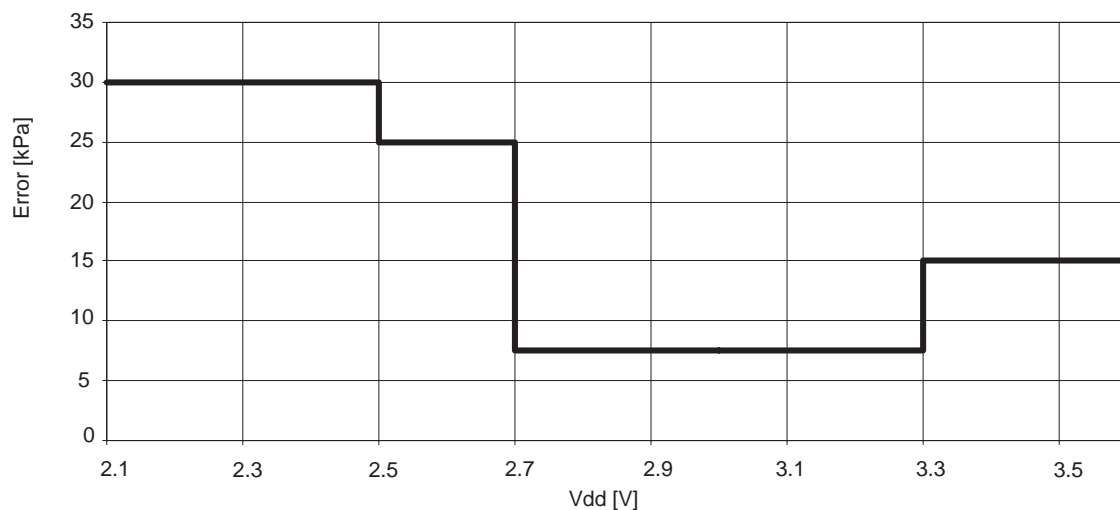
Figure 10. Pressure Error vs V_{DD} at 25^{\circ}\text{C} , 250 \text{ kPa} \leq P \leq 450 \text{ kPa}
