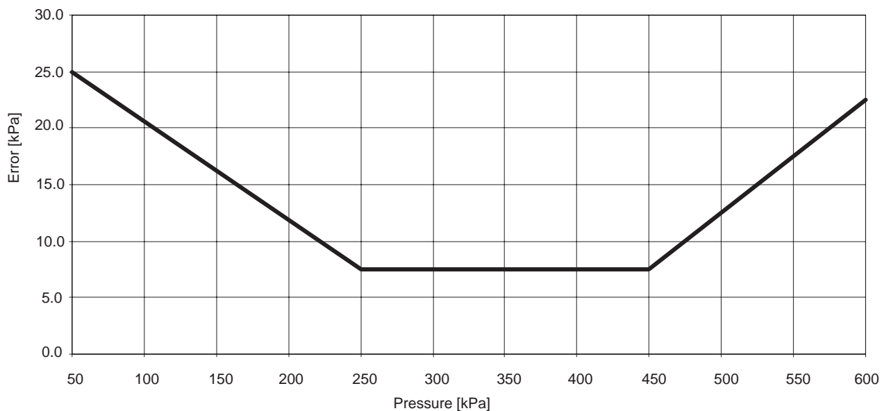
Figure 9. Pressure Error vs Pressure at T = 25^{\circ}\text{C} , 2.7 \leq V_{DD} \leq +3.3 \text{ V}
